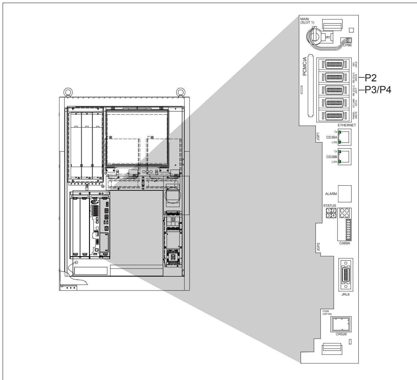
Figure 14-4. Location of Ports on the Controller
