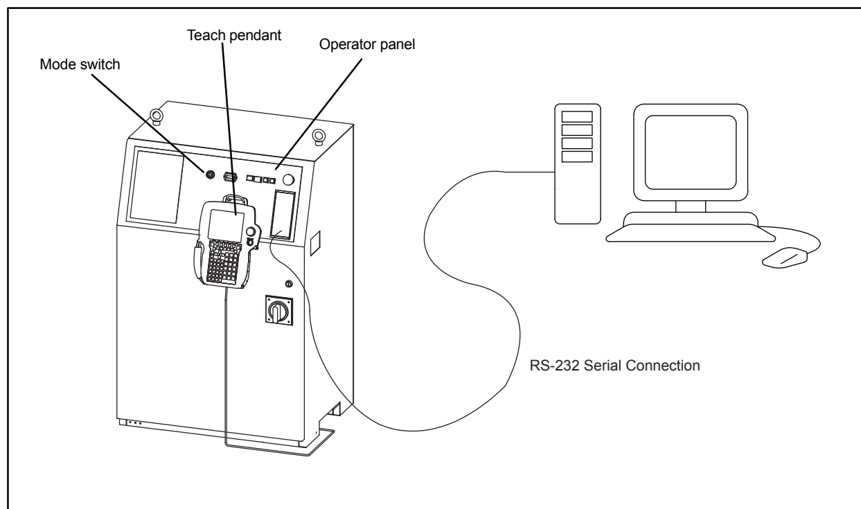
Figure 1–2. R-30iA Controller
