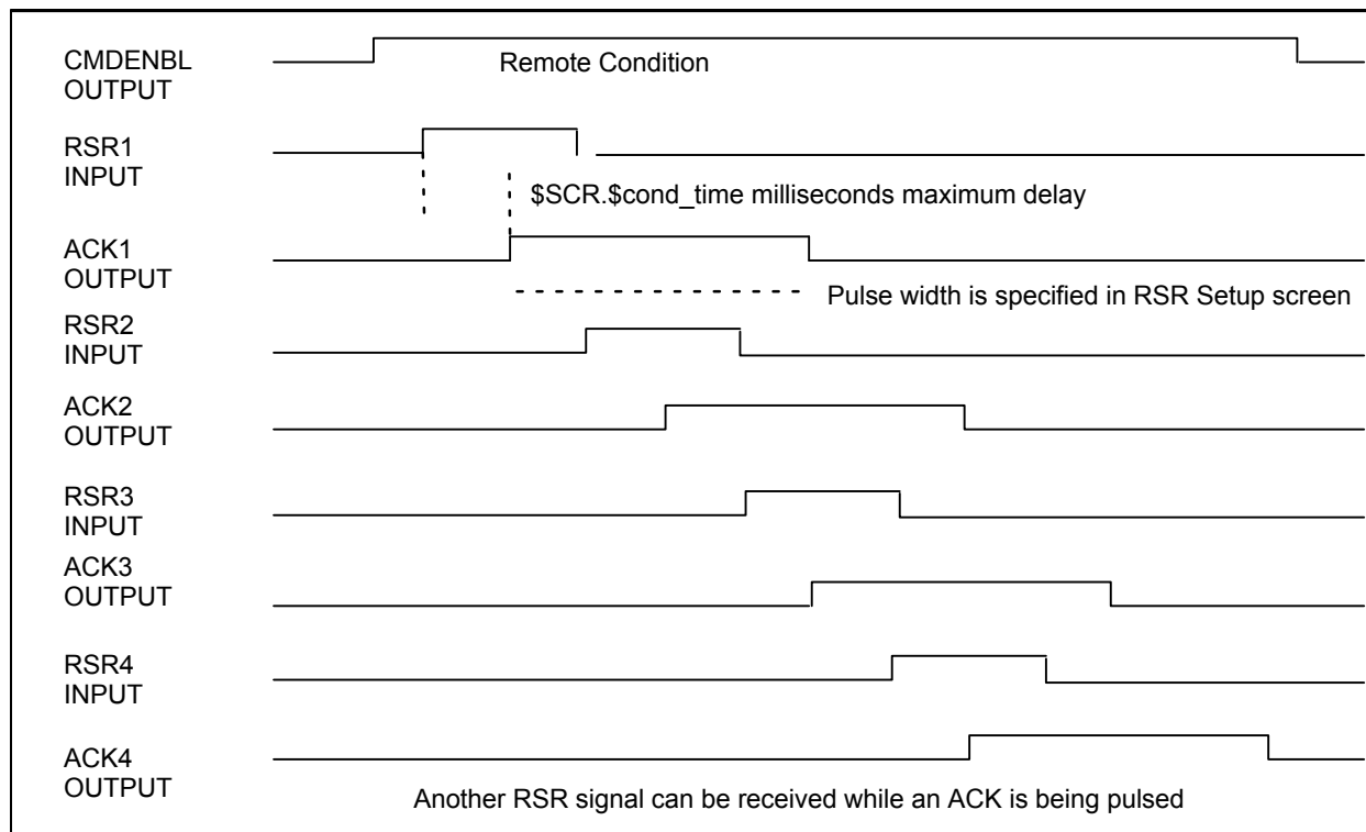
Figure 14–2. RSR Timing Diagram
